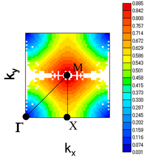
Fig.6 EFS of phononic crystal consisting of tungsten cylinders in water. (filling fraction f=0.5 )
