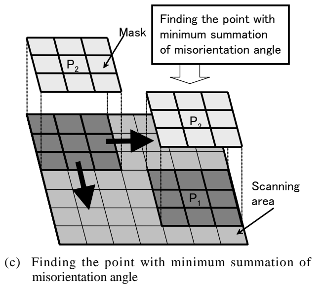
Fig. 4 Explanation of the method to determine the same point before and after fatigue testing.
