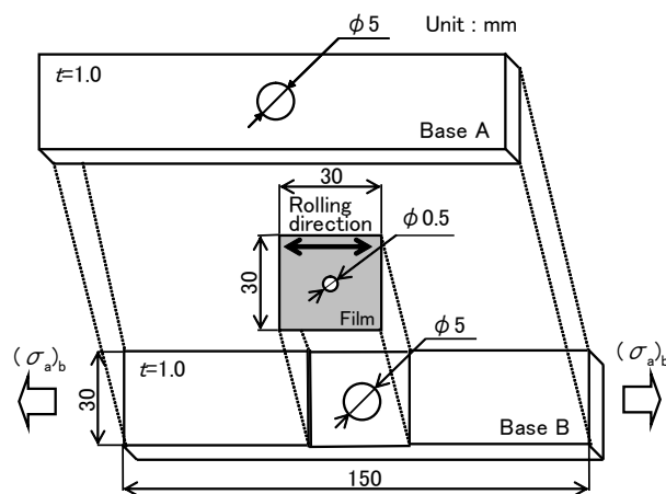
Fig. 2 Dimension of the film fatigue specimen.
