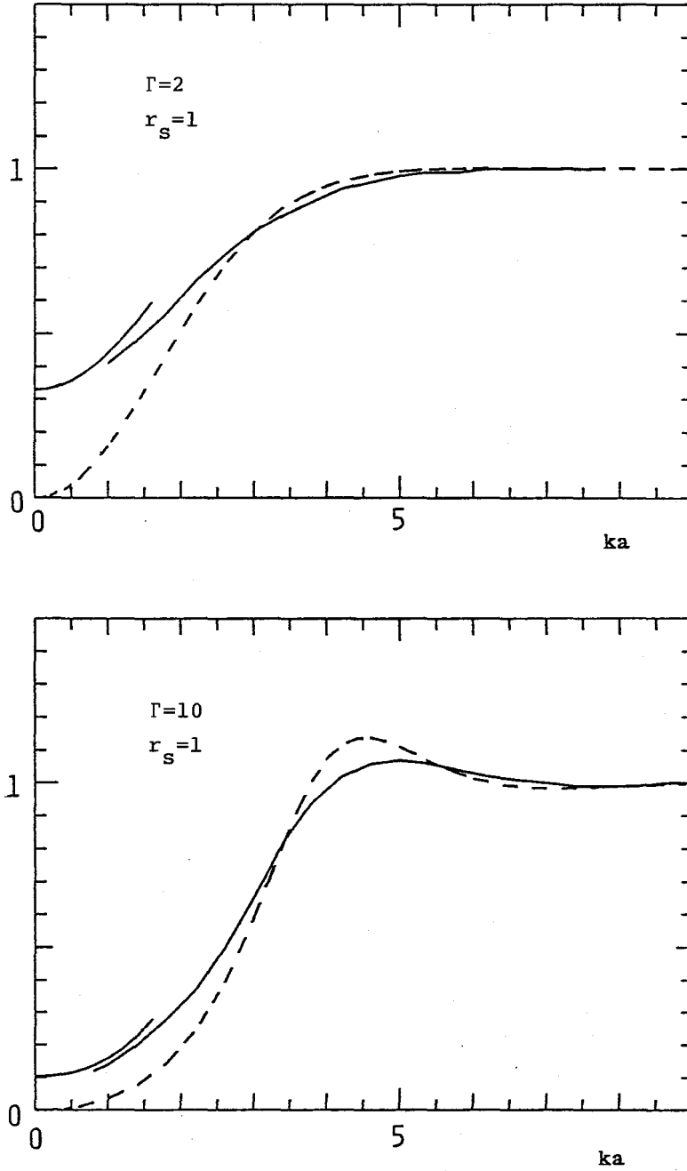
Fig. 5. The structure factor of ions in polarizing background of electrons with r_s=1 (solid lines), in comparison with the case of the one-component plasma (broken lines).
