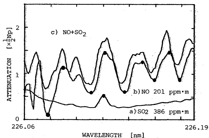
Fig.4 Absorption spectra of (a) sulfur dioxide, (b) nitric monoxide, and (c) their mixture.
