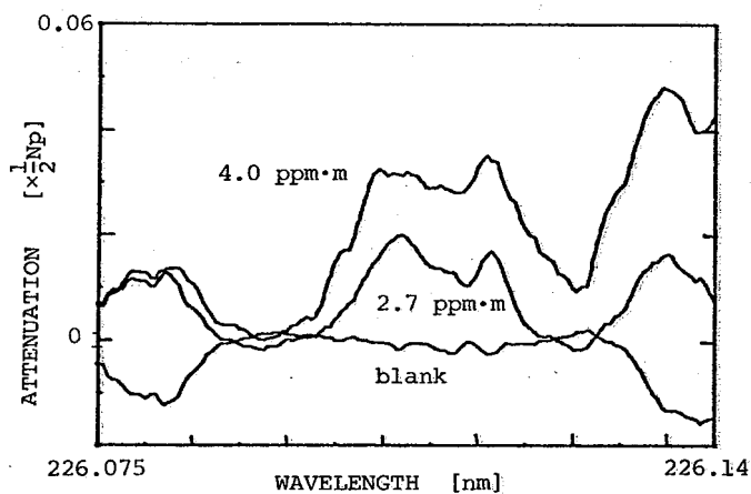
Fig.3 Absorption spectra of very dilute nitric monoxide.
