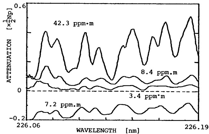
Fig.1 Absorption spectra of nitric monoxide in \gamma -0 band taken by the test system.
