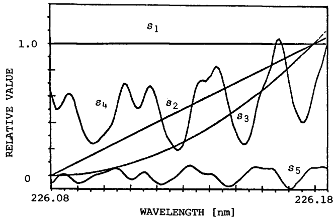
(a) base spectra
