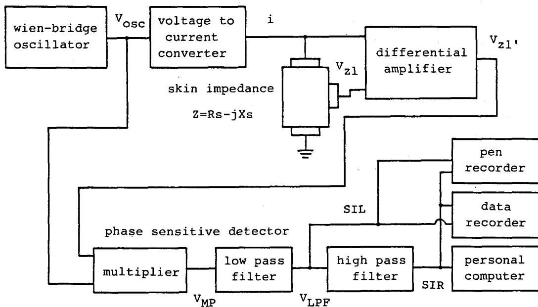
Fig.1 Block diagram of GSR measurement system.
