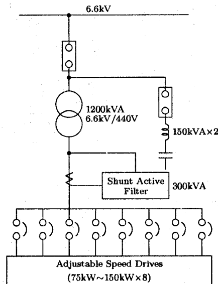
Fig. 7. Application to harmonic compensation
