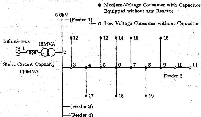
Fig. 11. Radial distribution system in residential area
