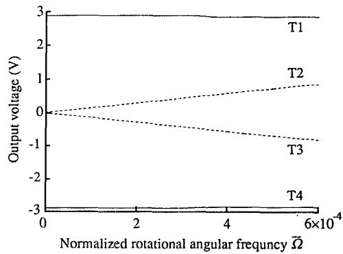
The normalized figure of merit \eta = 0.82
