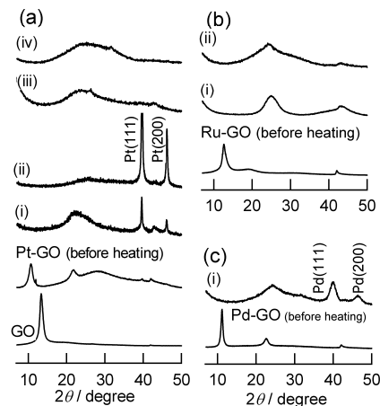
Fig. 2 X-ray diffraction (XRD) patterns of raw materials and heated samples: (a) GO and Pt-GO (before heat treatment), and the latter Pt-GO heated at 573 K (i), 673 K (ii) in air, 573 K (iii), 673 K (iv) in N_2 ; (b) Ru-GO (before heat treatment) and Ru-GO heated at 573 K (i), 673 K (ii) in N_2 ; (c) Pd-GO (before heat treatment) and Pd-GO heated at 673 K (i).
