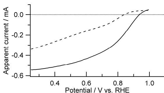
Fig. 4 Hydrodynamic voltammograms at 900 rpm under an oxygen atmosphere of Pt-GO heated at 673 K in air (solid line) and Pd-GO heated at 673 K in N 2 (broken line).
