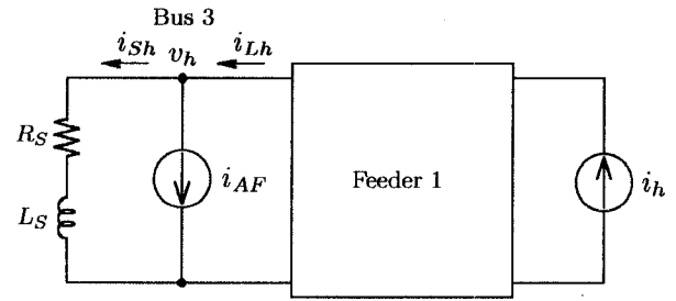
Fig. 9. Equivalent model for voltage and current harmonics.
