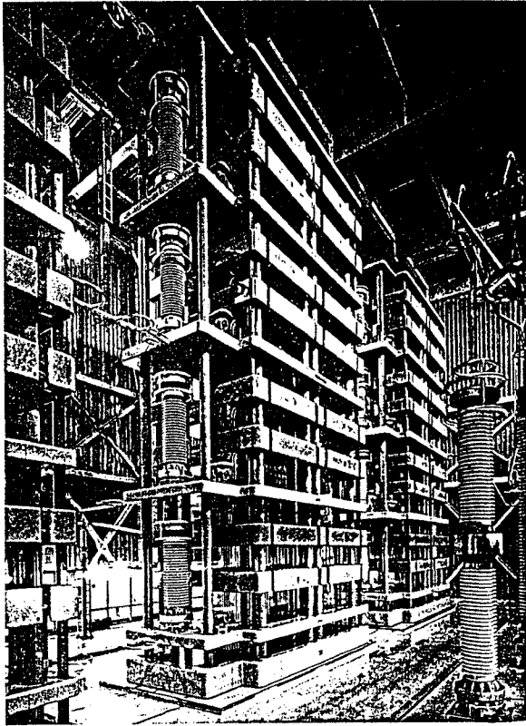
Fig. 5. Thyristor valve used for the 250-kV, 1.2-kA HVDC transmission system.
