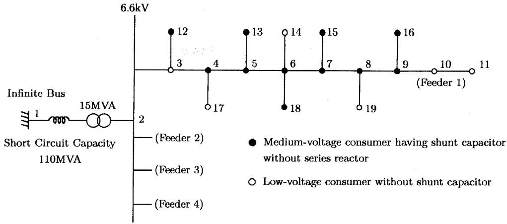
Fig. 8. Radial distribution system model.
