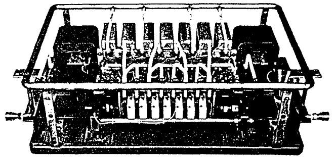
Fig. 4. Thyristor module for HVDC thyristor valves.
