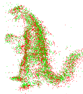
Figure 2: (a) One of the 36 frames of the test image sequence. (b) The sparsity pattern of the Hessian for decimated 100 points; nonzero elements are indicated in black. (c) The reprojection error e vs. the number of iteration. (d) The numerical value of e at each iteration. (e) 3-D reconstruction. Red: initial positions. Green: final positions.
