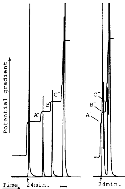
Fig. 3. Withdrawal of a target component. Equal volumes of 0.01 M solutions of citrate, lactate, and succinate were mixed and 9 \mu l of the resultant solution analyzed under the conditions in Table 1. The result is on the left.
