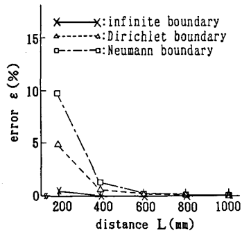
(a) accuracy
