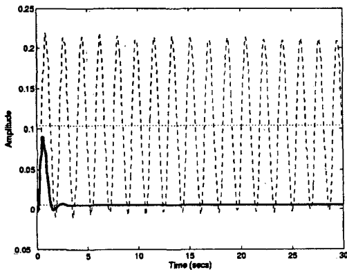
Figure 3: Step response of the plant in open and closed loop
