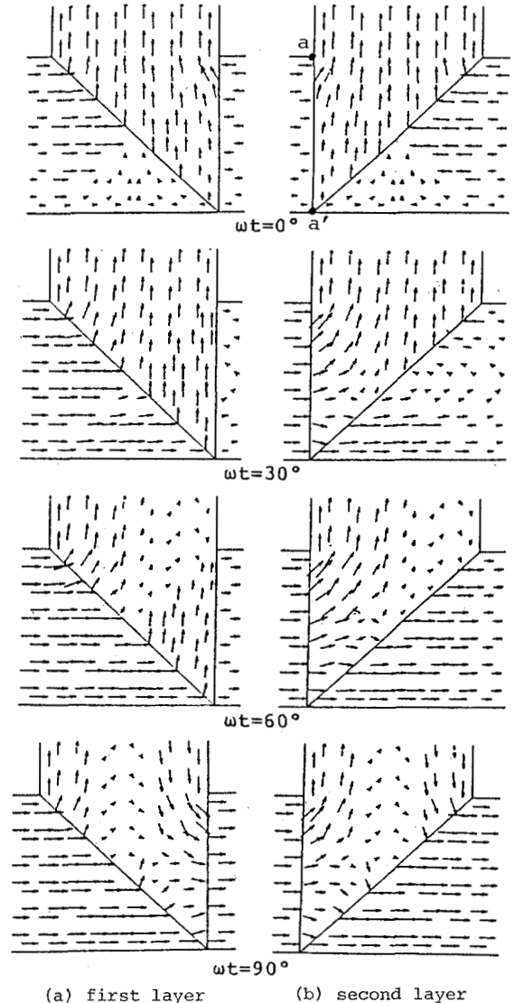
Fig.4 Flux density vectors in each layer (M-5, 0.35mm, Bleg=1.7T).
