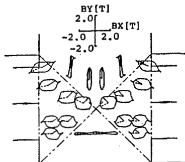
Fig.7 Loci of the apparent flux density vectors (M-5, 0.35mm, Bleg=1.7T).
