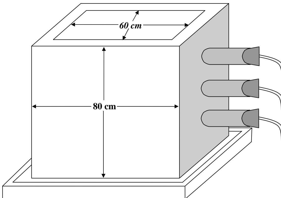
Fig. 1 Design of concrete tank used for the simulation study
