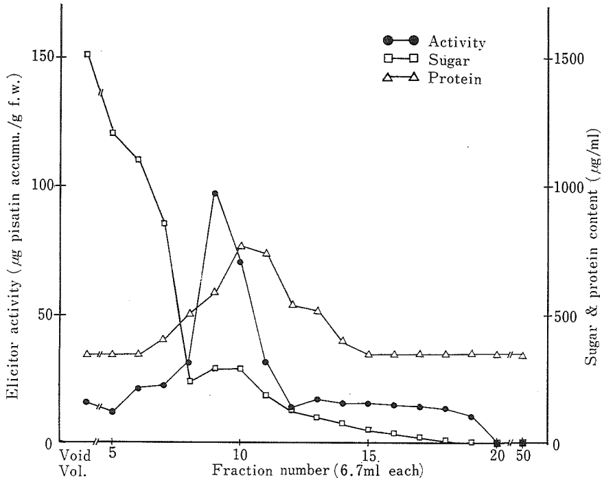
Fig. 1 Elution profile of elicitor activity, sugar, and protein of high molecular weight fraction from spore germination fluid of M. pinodes through Sephadex G-200 column.
