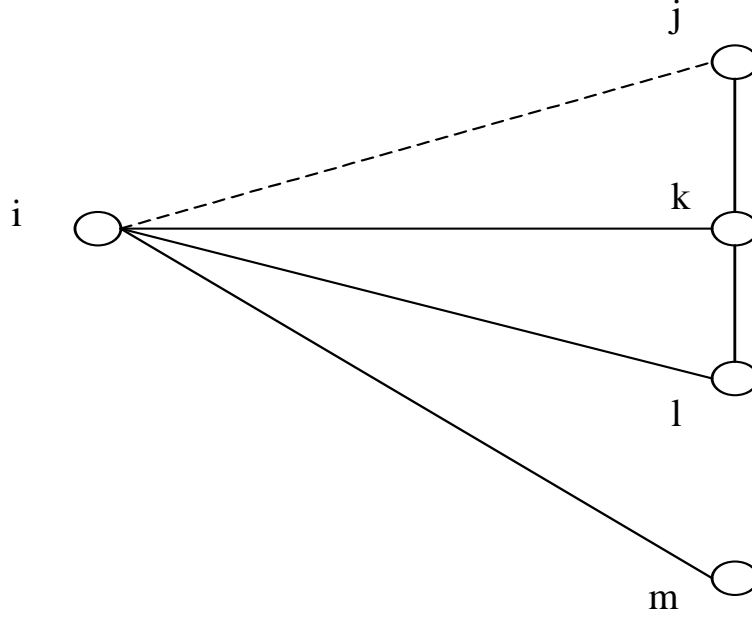
Figure 3: Stability in an Example Network
