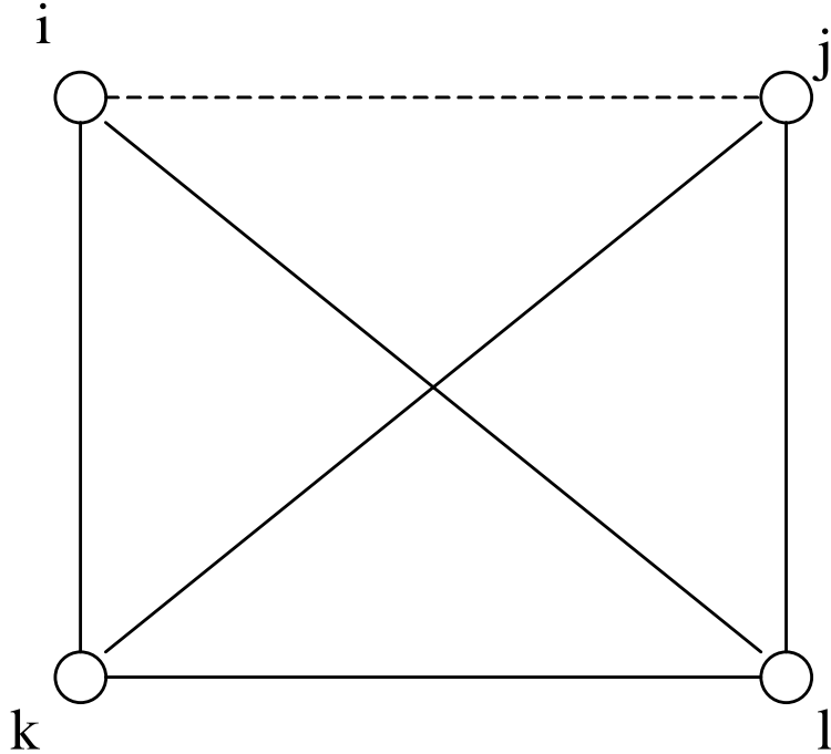
Figure 5: Stability in the Complete Network
