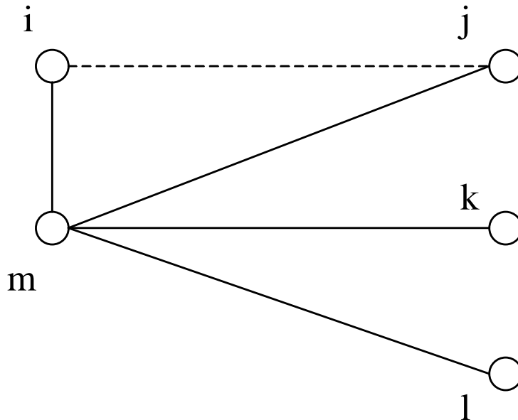
Figure 4: Stability in the Star Network
