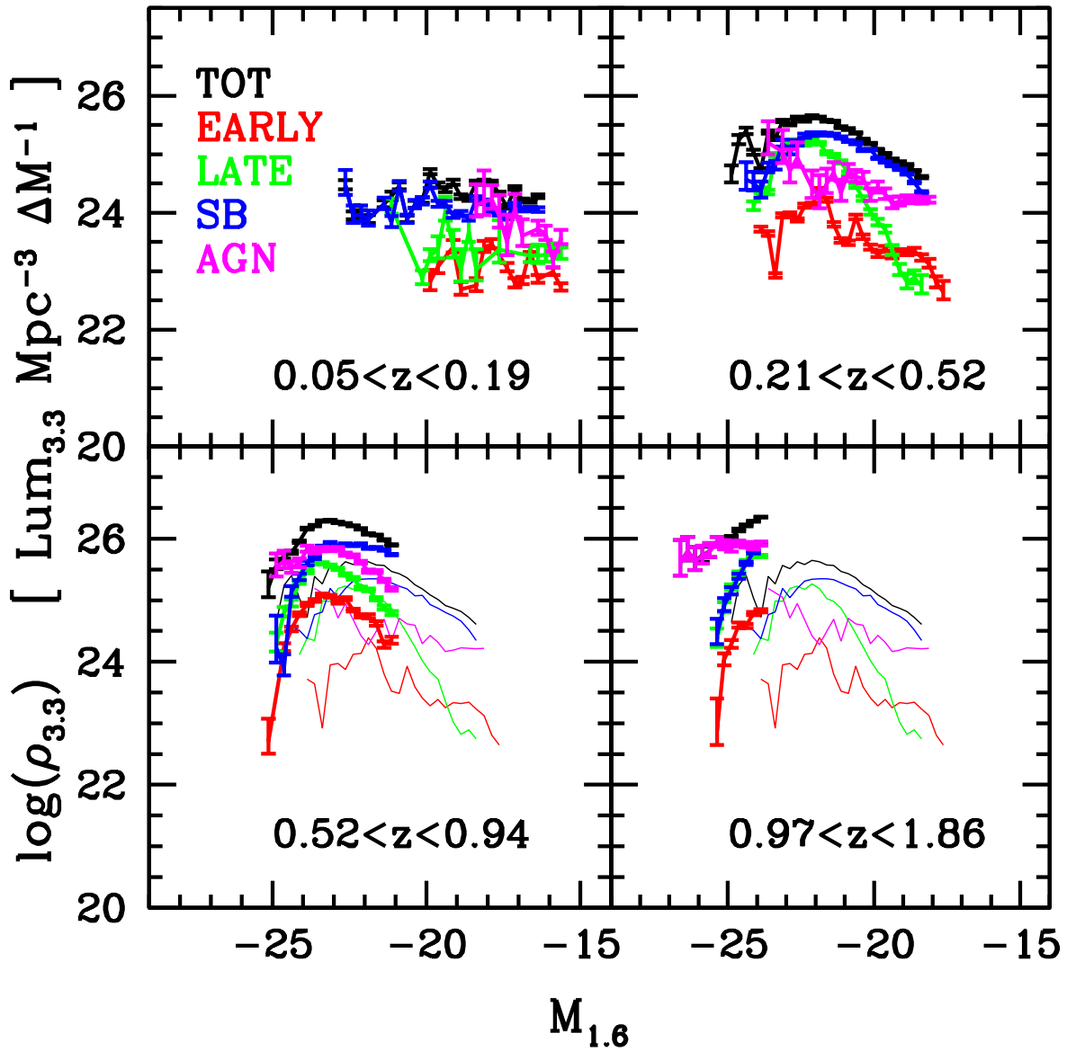
Figure 4.15: Rest-frame 3.3 \mu\text{m} dust LDFs depending on distance and galaxy type: Total population (black), Early (red), Late (green), Starburst (blue), and AGN (magenta). Due to the irregular trends in the low redshift panel, the trend shown by each galaxy population in the 0.21 < z < 0.52 redshift panel is displayed instead in the subsequent panels for comparison. The dust LDFs were trimmed according to the cuts adopted in Figure 4.9.
