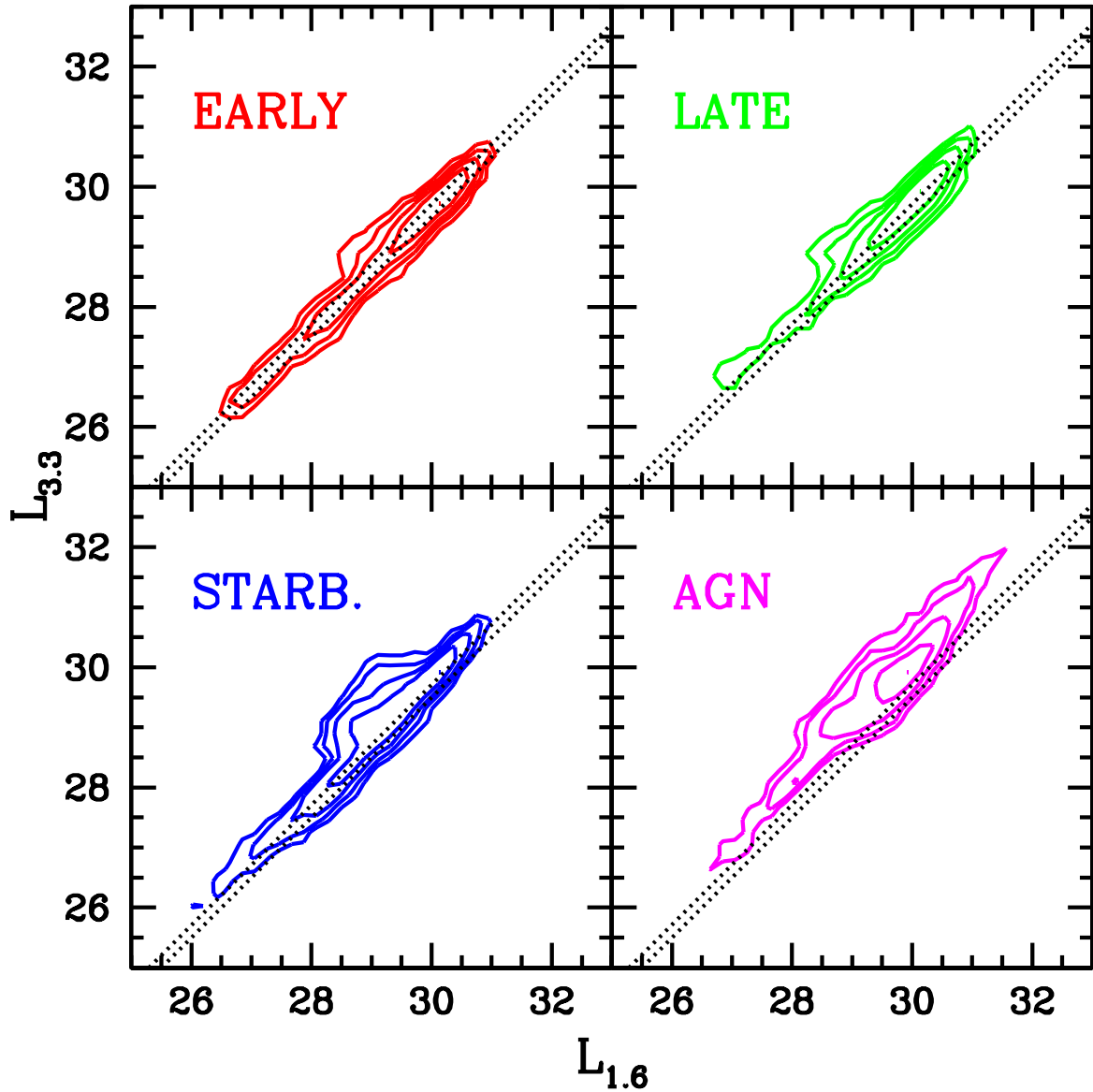
Figure 4.7: Luminosities at rest-frames 1.6 \mu\text{m} ( L_{1.6} ) and 3.3 \mu\text{m} ( L_{3.3} ). The dotted lines delimit the region where pure stellar emission should fall. Each panel is reserved to a different population: early-type (upper left), late-type (upper right), starburst (lower left), and AGN host (lower right). The contours are simply demonstrative of the sample distribution and are defined based on the maximum source density in each plot, hence the isocontour levels differ between panels.
