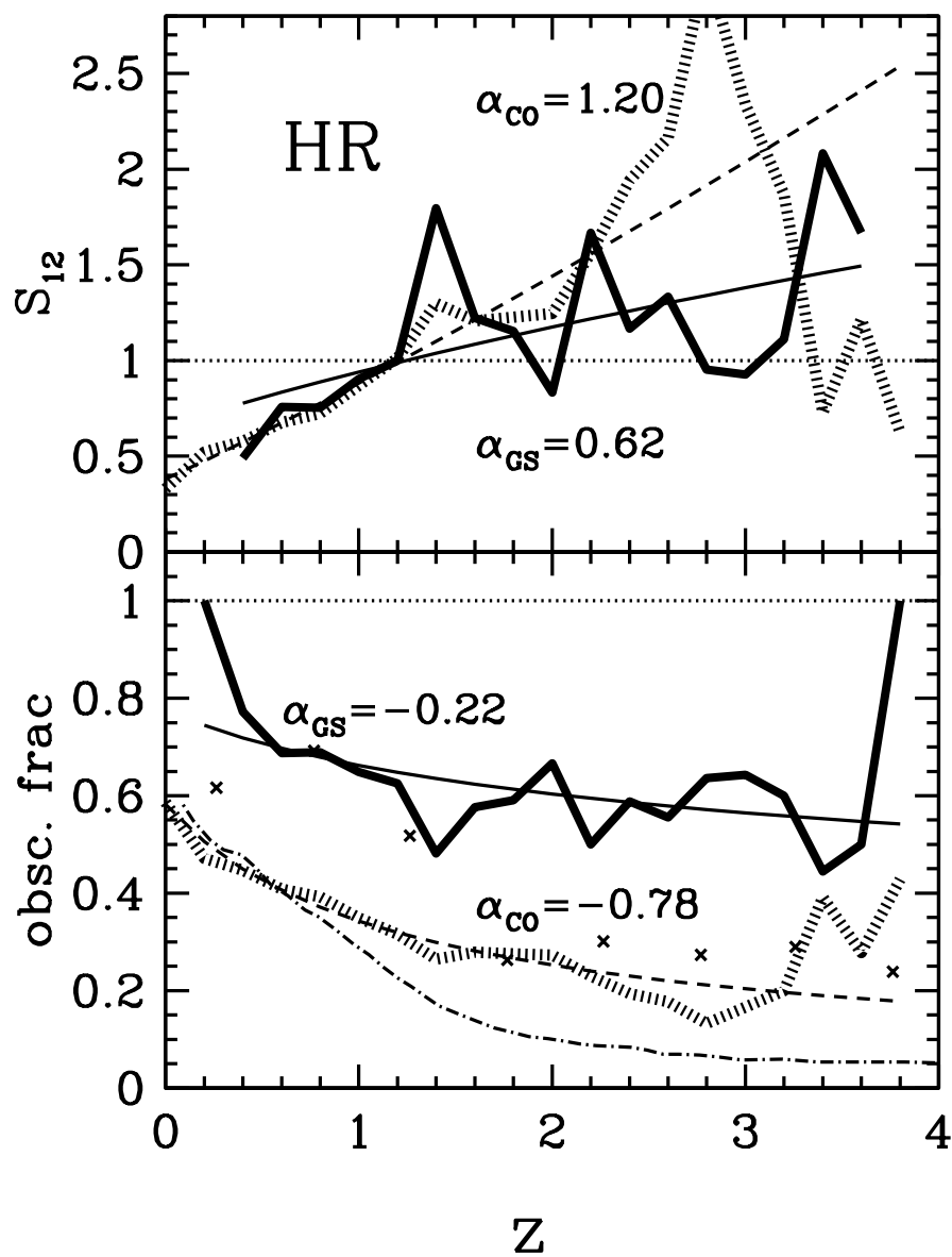
Figure 3.17: The same as in Figure 3.16, but considering the HR to identify obscured and unobscured sources instead of N_{\text{H}} and optical/nIR spectroscopy. Symbols and labelling as in Figure 3.16.
