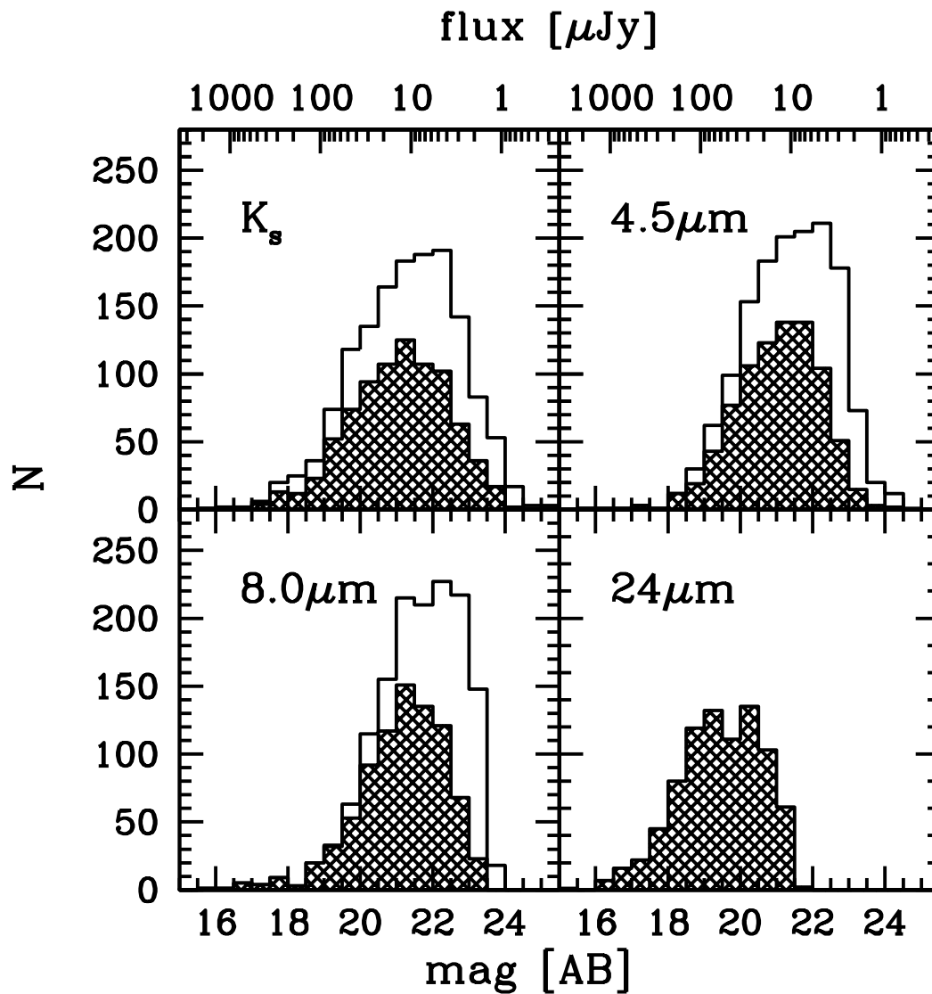
Figure 3.9: The distribution in magnitude of the final GOODSs sample with reliable photometry in K-IRAC bands (open histogram) and K-IRAC-MIPS 24 \mu\text{m} (hatched histogram). Each panel refers to the magnitude distribution in the following bands: K_s (upper left), 4.5\mu\text{m} (upper right), 8.0\mu\text{m} (lower left), and 24\mu\text{m} (lower right). Note that in the latter both histograms coincide.
