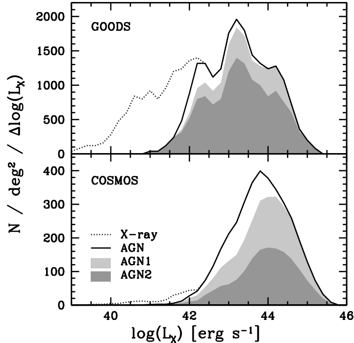
Figure 3.13: The source density distribution with intrinsic X-ray luminosity distribution for GOODSs (upper panel, \sim 140 arcmin ^2 ) and COSMOS (lower panel, 1.8 deg ^2 ) samples (note the y-axis are different). The trends were obtained with a moving bin of width \Delta \log(L_X) = 0.6 , with measurements taken each \Delta \log(L_X) = 0.2 . The overall X-ray population is represented by the dotted line, the AGN by the continuous line. The AGN population is further separated into type-1 (light shaded region, N_H(\text{cm}^{-2}) \leq 22 ) and type-2 (dark shaded region, N_H(\text{cm}^{-2}) > 22 ) sub-populations.
