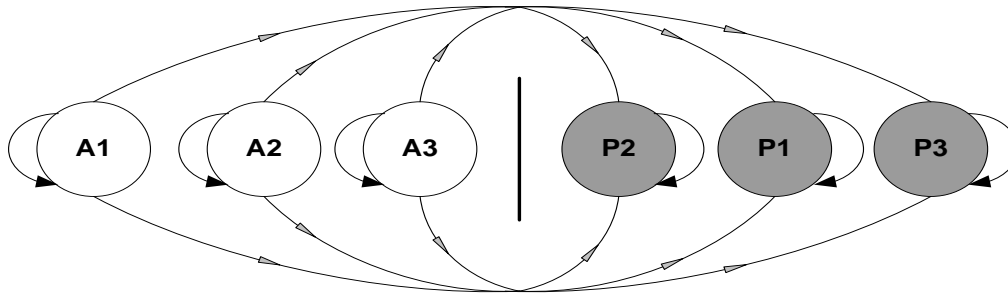
Figure 3. Simplified graph of the six-state model
