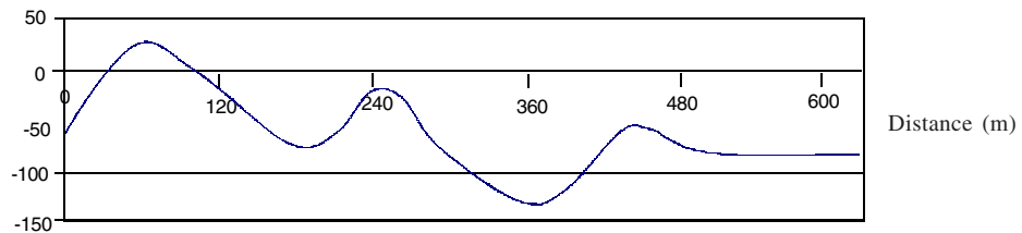
Figure-4.1d : Total Relat Mag Intensity along Traverse 13 (S - N) of Ijeda - Iloko area
