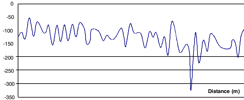
Figure-4.1c : Total Relat Mag Intensity along Traverse 9 (SE - NW) of Ijeda - Iloko area
