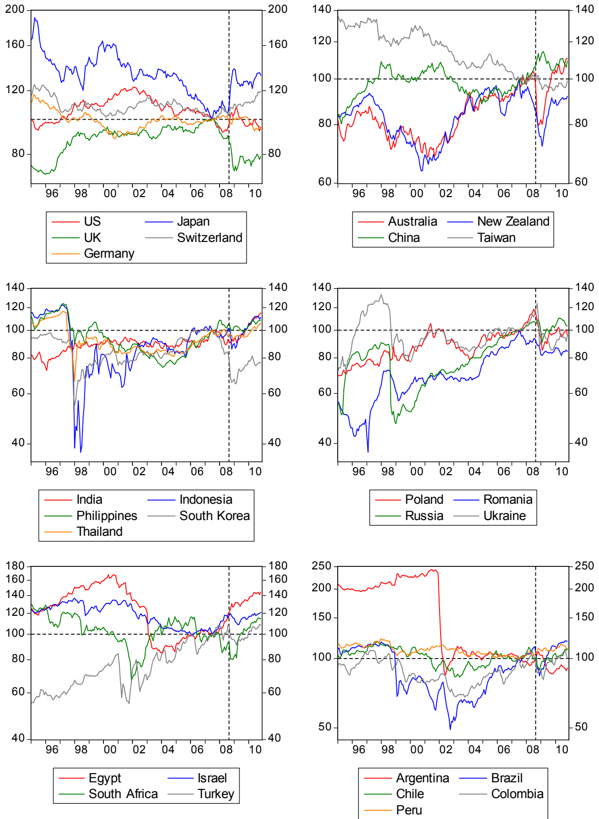
Figure 1: Real effective exchange rates based on consumer prices (January 1995=100), January 1995 - November 2010
