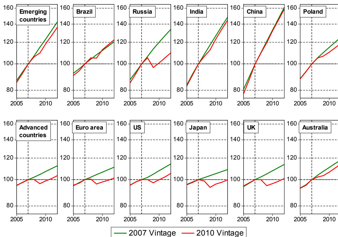
Figure 5: GDP forecasts to 2012: October 2007 versus October 2010 (2007=100)
