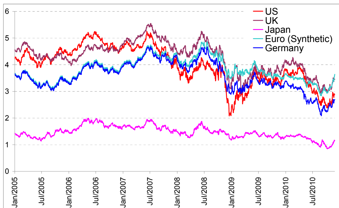
Figure 7: 10-year benchmark government bond yields, 3 January 2005 – 29 November 2010
