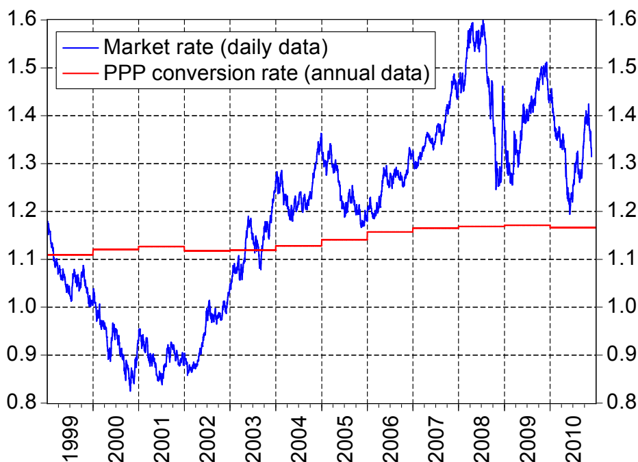
Figure 3: Exchange rate of the euro against the US dollar and the purchasing power parity (PPP) conversion rate, 4 January 1999 – 29 November 2010
