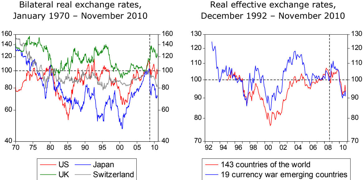
Figure 4: External real exchange rate of the euro (January 1995=100)
