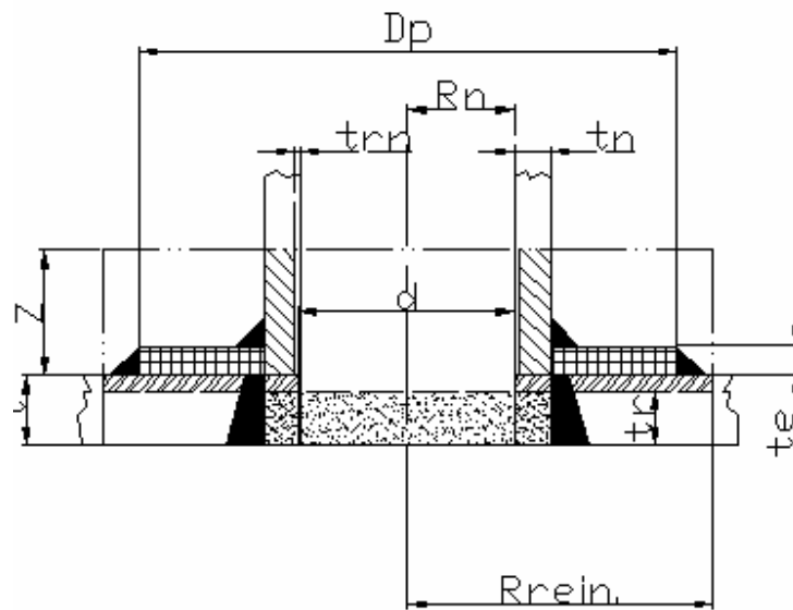
Gambar 4.3 Reinforcements Inlet-outlet Opening
