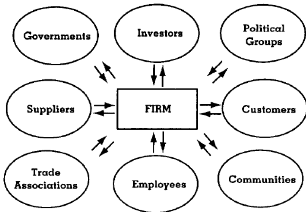
Figure 1: Stakeholder Theory
