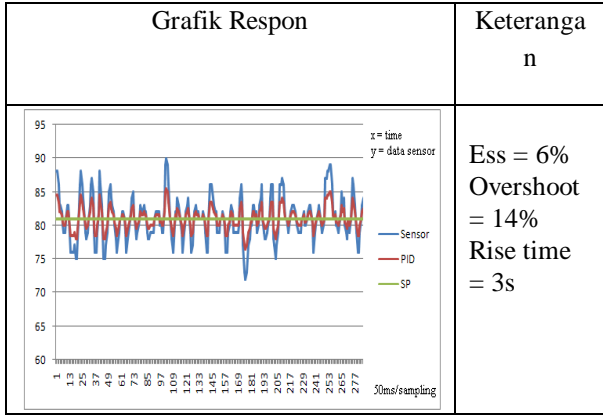
Gambar 11. Hasil Sinyal K_p=5, K_d=810, K_i=0.007
