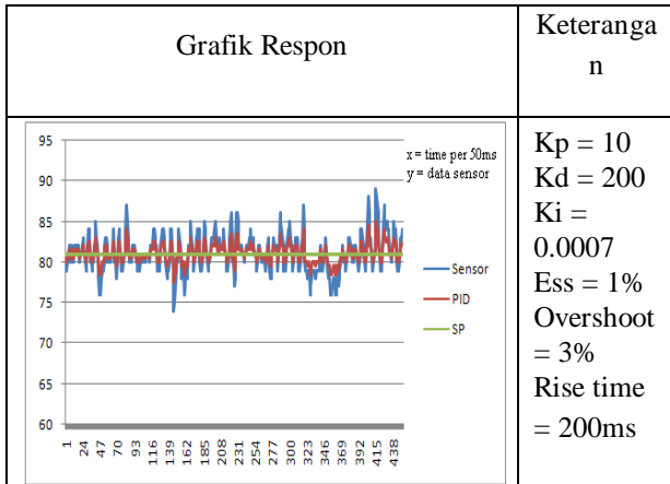
Gambar 12. Hasil Plot Sinyal PID trial and error
