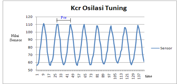
Gambar 9. Sinyal Osilasi (50ms/sampling)
