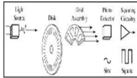
Gambar 3.2.1 rotary encoder
