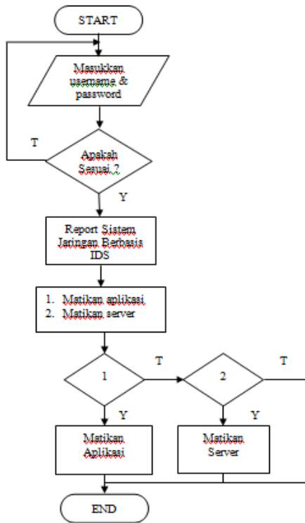
Gambar Flowchart Sistem
