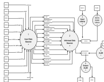
Gambar1. Context Diagram
