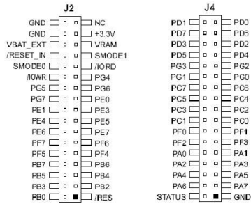
Gambar 2.1 Prototyping Board Pinout
