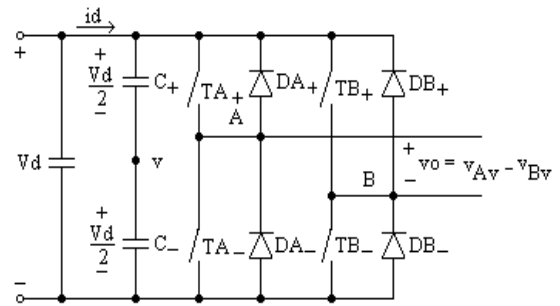
Gambar 4. Rangkaian full bridge inverter
