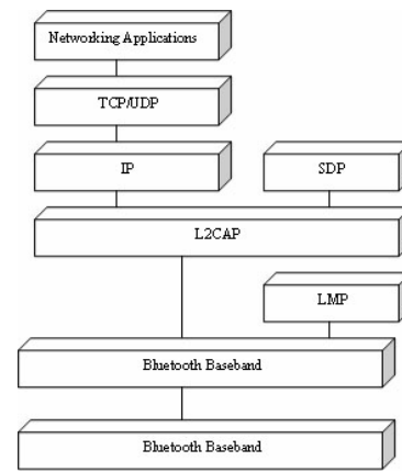
Gambar 2. BNEP stack[9]
