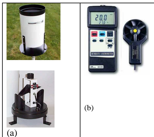
Gambar 2. Peralatan sensor a. Typing bucket rain gauge b. Anemometer Model AM420
