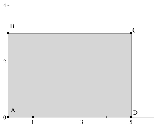
Figure 2. Rectangle ABCD
