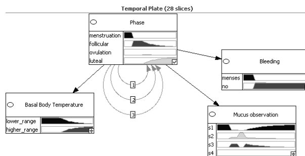
Figure 2: An example of third-order DBN model of woman's monthly cycle
