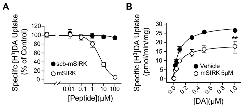
Figure 6. Activation of G\beta\gamma subunits reduces DAT activity in brain synaptosomes. (A) mSIRK reduces [ ^3 H]-DA uptake in rat striatal synaptosomes. Samples were pre-incubated for 10 min with various concentrations of mSIRK (open circles) or scb-mSIRK (filled circles) at 34°C, followed by the addition of [ ^3 H]-DA (final concentration, 0.1 \mu M) for 8 min, n=3. Nonspecific [ ^3 H]-DA uptake was determined in the presence of 10 \mu M nomifensine. (B) Kinetic analysis of the synaptosomal [ ^3 H]-DA uptake was determined in the absence (vehicle) or presence of 5 \mu M mSIRK, n=3. **p<0.01. doi:10.1371/journal.pone.0059788.g006
