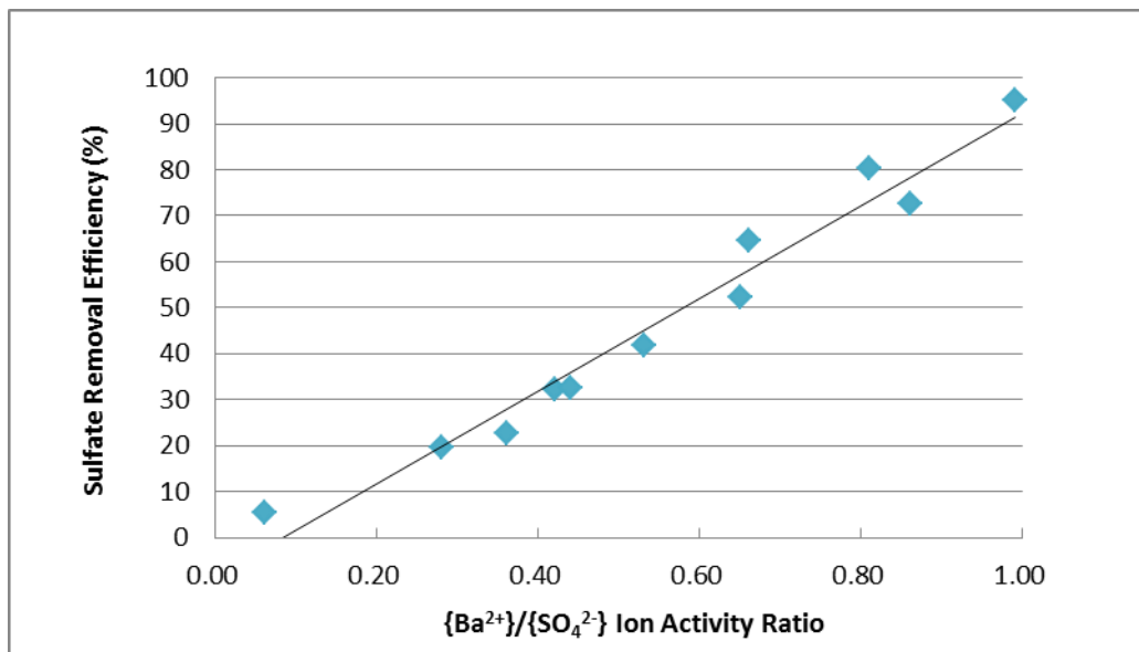
Figure 29. The correlation of {Ba 2+ }/{SO 4 2- } ion activity ratio with sulfate removal efficiency after 1 hour of contact time
