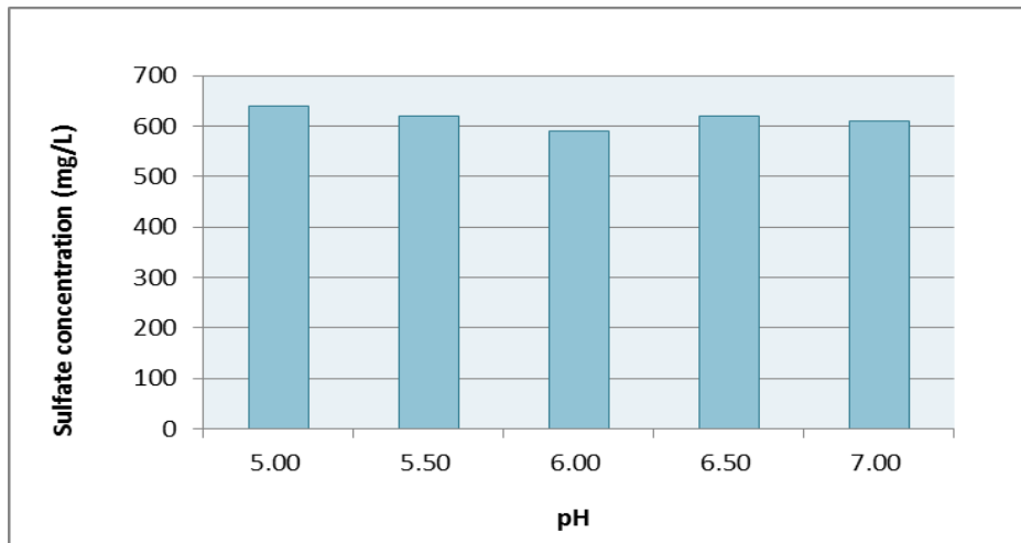
Figure 7. Impact of pH on effluent sulfate concentration in conventional flocculation process for Mixture 1
