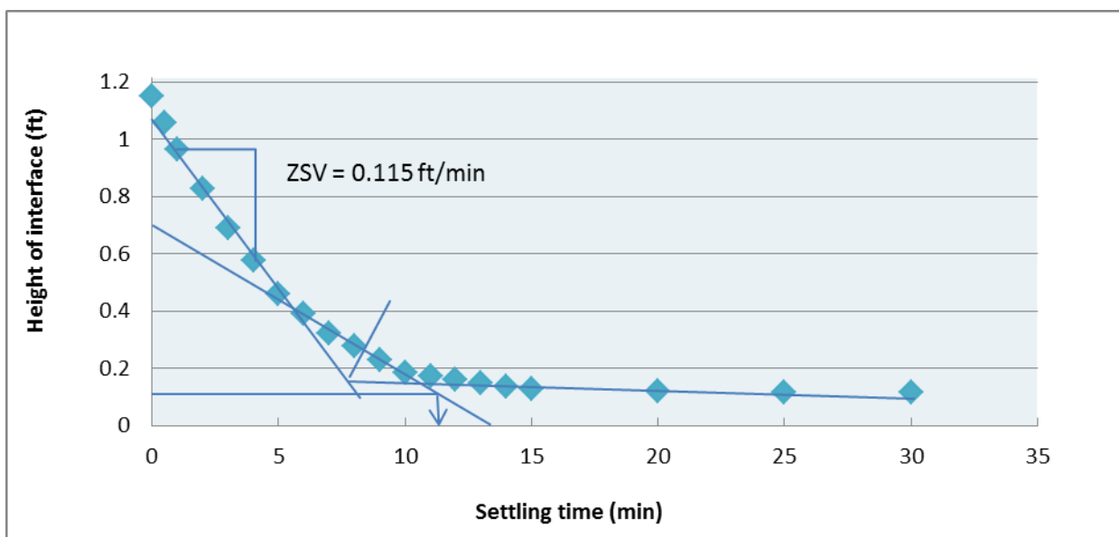
Figure 33. Settling curve of conventional flocculated sludge
