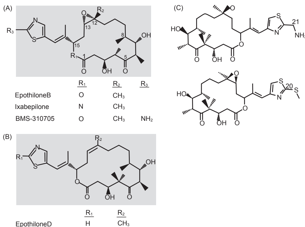
Figure 1 Chemical structures of the epothilones under clinical development. (A) Structure of epothilone B, ixabeplilone, and BMS-310705. (B) Structure of epothilone D. (C) Structure of epothilone D second generation. From Fumoleau P, Coudert B, Isambert N, et al. 2007. Novel tubulin-targeting agents: anticancer activity and pharmacologic profile of epothilones and related analogues. Ann Oncol , 18(Suppl 5):v9-15, by permission of Oxford University Press © 2007.
