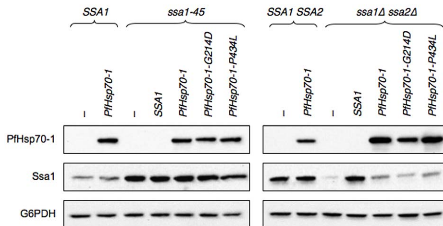
Figure 6. Ssa1 is not upregulated in response to wild type or mutant PfHsp70-1 expression. The indicated yeast strains transformed with the indicated plasmids were grown in liquid culture to log phase at 26°C and were then incubated at 37°C for 30 min. Equivalent amounts of cells were harvested, and samples were processed as described in the “Methods”. Note: The anti-Ssa1 antiserum crossreacts with Ssa3 and/or Ssa4, since there is a faint band in the ssa1Δssa2Δ strain transformed with the empty vector. This antiserum recognizes the last 56 amino acids in Ssa1 (E. Craig, personal communication). Also note that the levels of the PfHsp70-1 mutants are similar to the level of the wild type protein (compare the last three lanes, top-right panel). The absence of an increased level of Ssa1 in ssa1-45 yeast containing the SSA1 expression vector most likely results from the fact that the protein binds to its message and represses translation [71]. Thus, the expression of Ssa1 is expected to depress both its own synthesis and the synthesis of the Ssa1-45 mutant protein.
