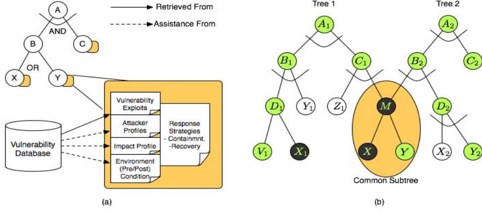
Fig. 3. (a) An AST with associated information (b) ASTs with a common sub-tree
