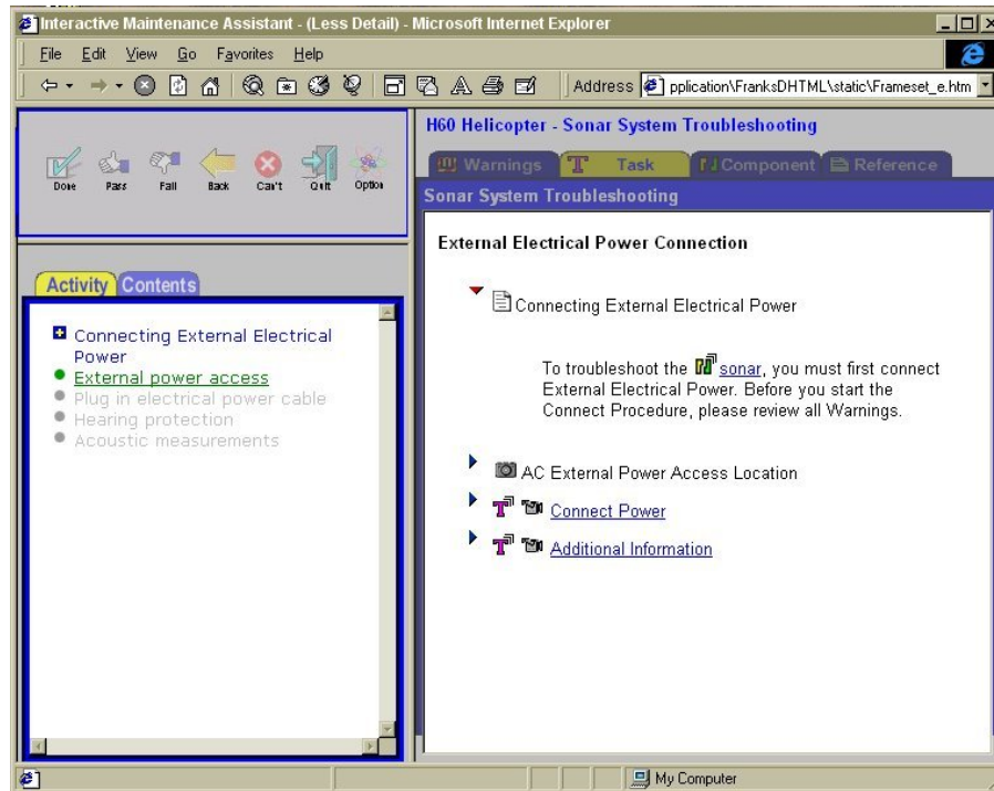
Figure 5. When presenting supporting information for a troubleshooting step, ADAPTS uses the stretched approach (right): depending on user goal and knowledge, fragments can be shown or hidden; however, the user can override system's selection.
