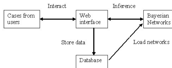
Figure 2: MARILYN’s architecture
