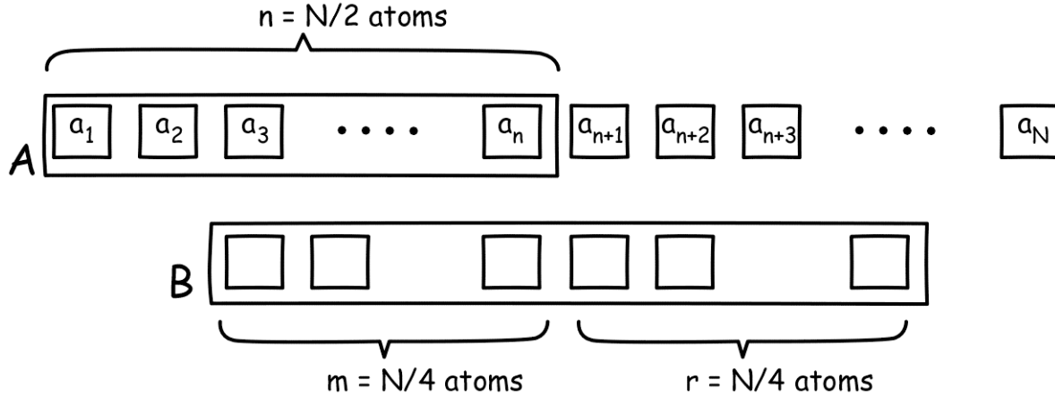
Figure 9. Most frequent distribution of atoms in propositions A and B
