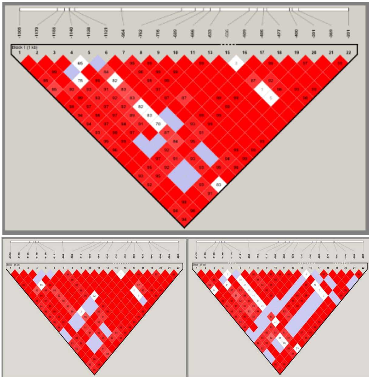
Figure 1: Haploview results
