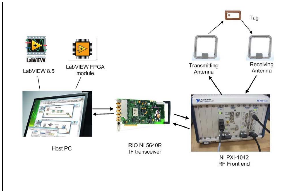
Figure 17. ISO 18000-3 Model 1 conformed transmitter-receiver system hardware structure
