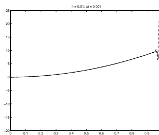
Figure 4: \Delta t = 0.001
