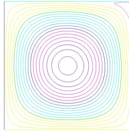
Figure 9: Computed solution \mathbf{u}_2^h , k = h = 1/32
