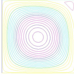
Figure 8: Computed solution \mathbf{u}_2^h , k = h = 1/16
