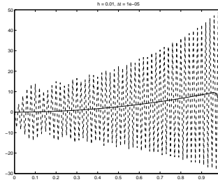
Figure 6: \Delta t = 0.00001
