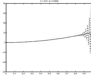
Figure 5: \Delta t = 0.0002
