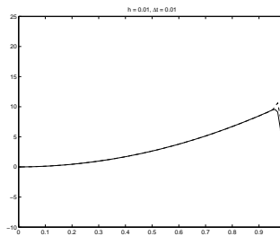
Figure 3: \Delta t = 0.01
