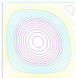
Figure 7: Computed solution \mathbf{u}_2^h , k = h = 1/8
