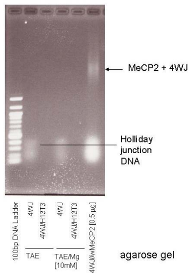
Figure 6. Gel shift.
