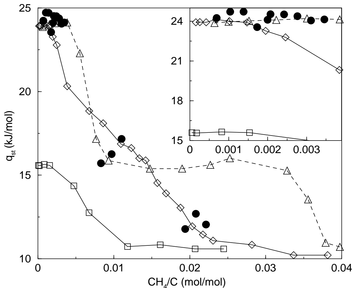
Figure 7.2: Isosteric heats of adsorption for CH_4 from experiments 34,37 (circles) and simulations. The diamonds (squares) are for adsorption onto heterogeneous (homogeneous) bundles. The triangles are for a homogeneous bundle with the solid-fluid potential increased by 45%. All bundles contain 45 nanotubes. The simulations were performed at 159.88 K. The inset shows q_{st} at low coverage. The lines are drawn as a guide to the eye. The estimated error bars are about the size of the symbols.
