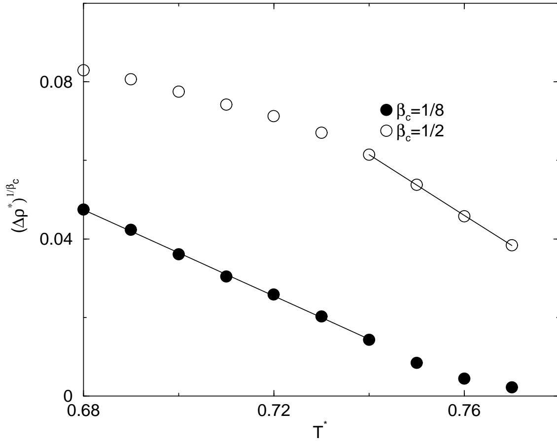
Figure 3.3: Scaled width of the coexistence data versus reduced temperatures for the capillary condensation of methane in a graphitic slit pore. The 2-D Ising exponent of \beta_c = 1/8 is shown as \bullet and \circ denotes the mean-field value of \beta_c = 1/2 .
