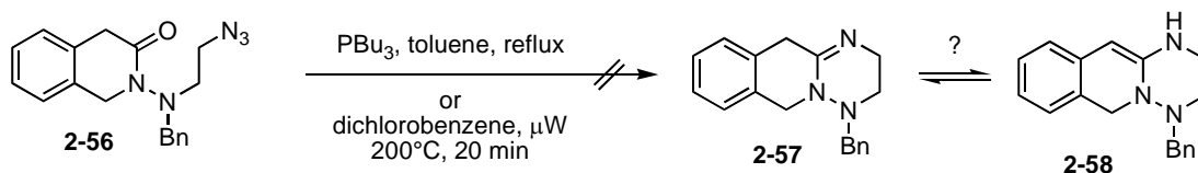
Scheme 2-12. Screening the SAW reaction conditions on substituted lactams
