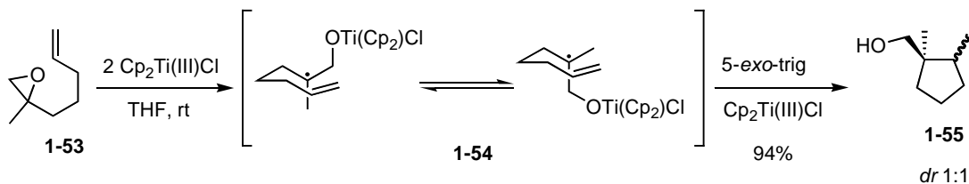
Scheme 1-13. Synthesis of cyclopentanol 1-55 using titanocene(III) chloride
