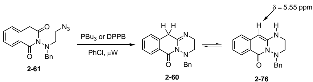
Scheme 2-18. Staudinger/ aza -Wittig then oxidation approach
