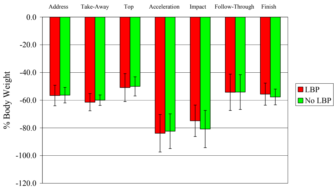
Figure 4.3 Compressive forces (at L5/S1) at 7 swing points
