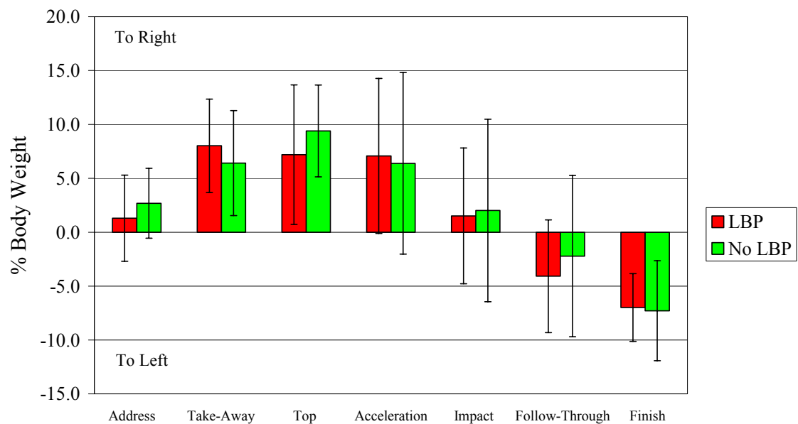
Figure 4.2 Right-left shear forces (at L5/S1) at 7 swing points
