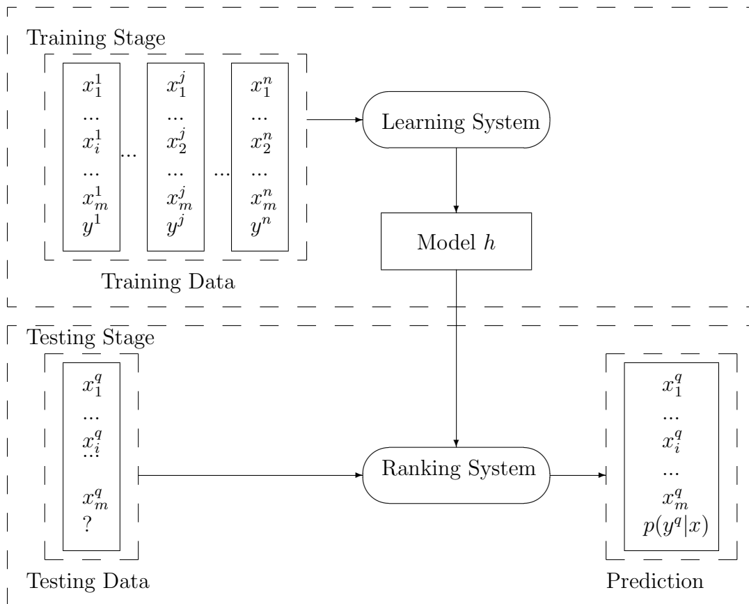
Figure 7: The learning to rank framework
