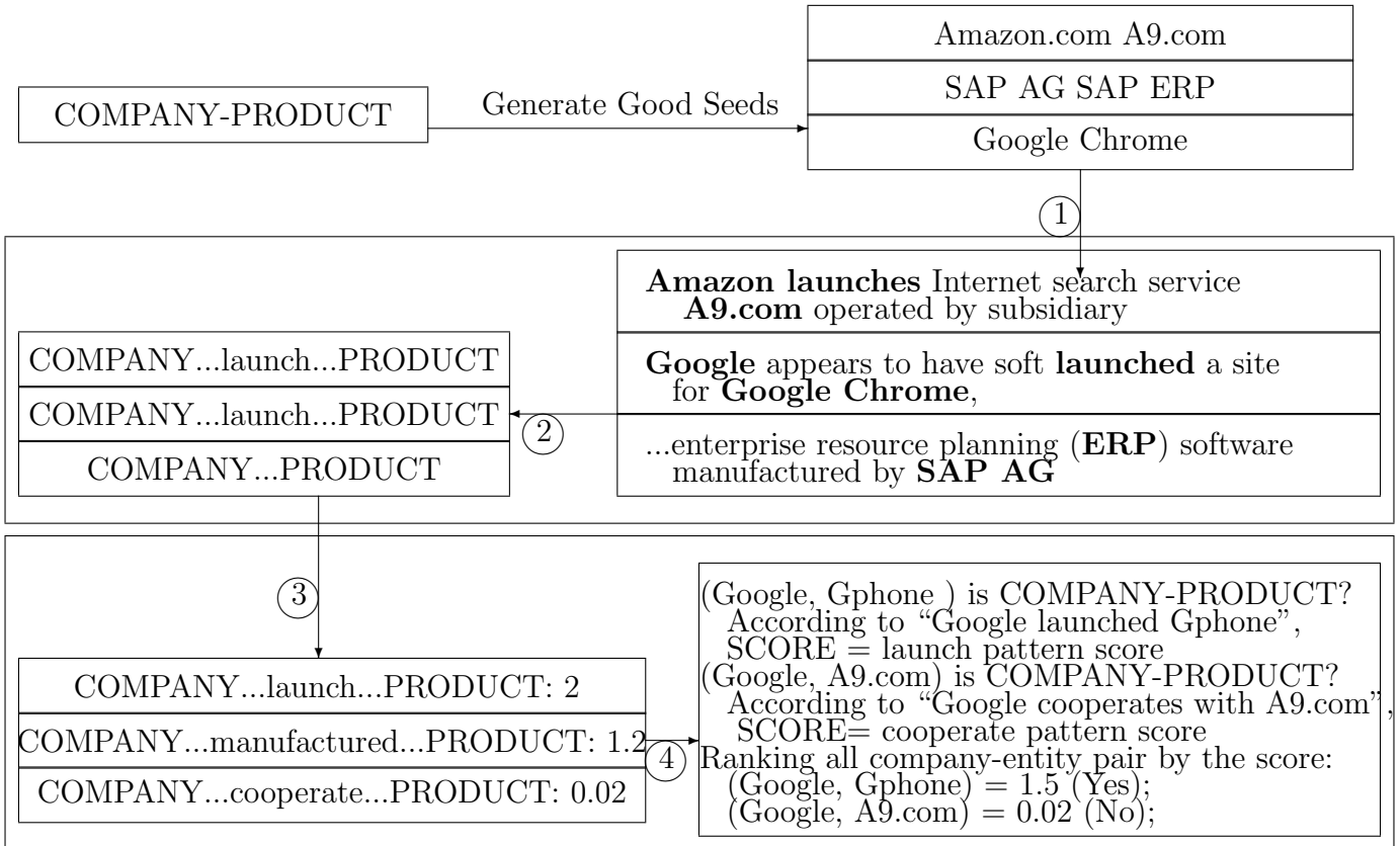
Figure 11: Bootstrap framework of topic-answer entity pair extraction
