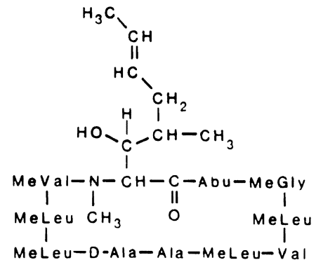
Fig 1. Structural formulas of FK 506 and CyA.
